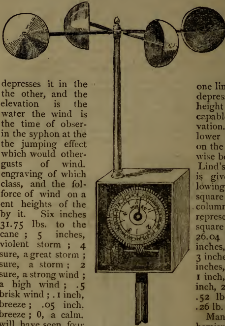
WIND GAUGE.
